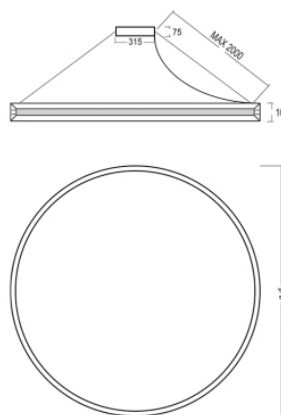
Technical drawing: OUSE SUSPENDED
